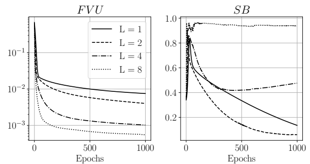
Figure 5: Experiment 4: Resulting FVU and spectral bias for NNs with varying number of layers L = 1, 2, 4, 8 when learning f_2(x) .
