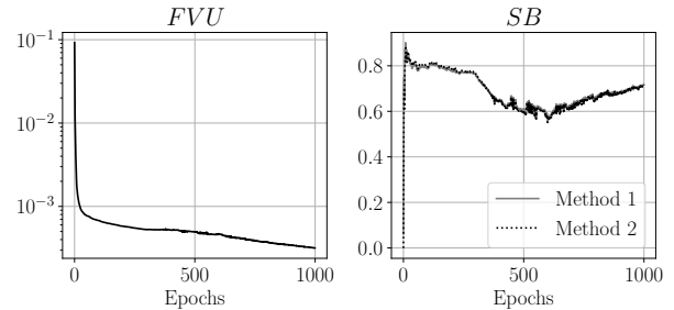
Figure 2: Experiment 2: Resulting FVU and spectral bias for a ReLU network trained to regress the target f_2(x) using Method 1 and Method 2 respectively. Both methods produce similar results.
