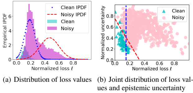
Figure 2: Loss values and epistemic uncertainty distribution on CIFAR-10 with 90% symmetric noise, a warm-up of 30 epochs. (a) Loss distribution of clean samples overlaps with noisy samples due to misleading predictions accompanied by a high level of epistemic uncertainty. (b) Label noise modeling considering epistemic uncertainty distinguishes clean samples from noisy ones more accurately.
