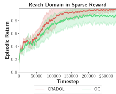
Figure 7: In domains with small or negligible context-specific abstraction, the benefit of CRADOL is not as significant compared to the Reacher domain, where the low-dimensional observation representation does not require context-specific abstraction. This figure shows the mean and 95% confidence interval computed for 10 seeds.
