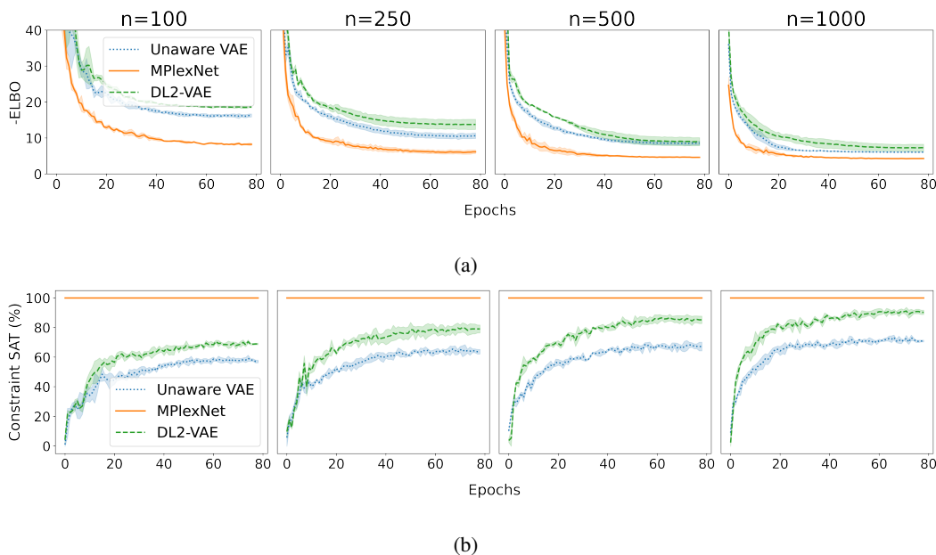
Figure 3: Results from the synthetic data experiment (a) Negative lower bound to the held out likelihood of data (-ELBO). The MultiplexNet approach learns to represent the data with a higher likelihood, and faster than the baselines. (b) % of reconstruction samples from the VAE that obey the domain constraints. The MultiplexNet approach, by construction, can only generate samples within the specified constraints.
