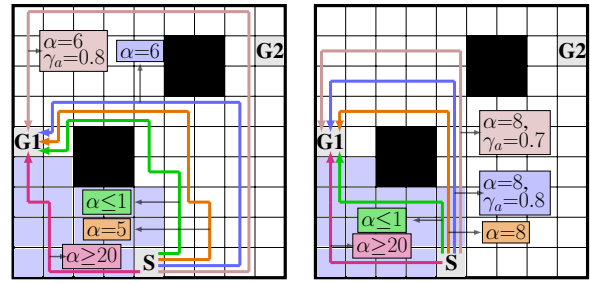
Figure 2: An illustration of deceptive trajectories generated by the proposed approach under various efficiency parameters ( \alpha ) and discount factors ( \gamma_a ). The agent starts from the state S . The true goal and decoy goal are G1 and G2 , respectively. \gamma_a = 1 if it is not written explicitly. (Left) Exaggeration behavior. (Right) Ambiguity behavior.
