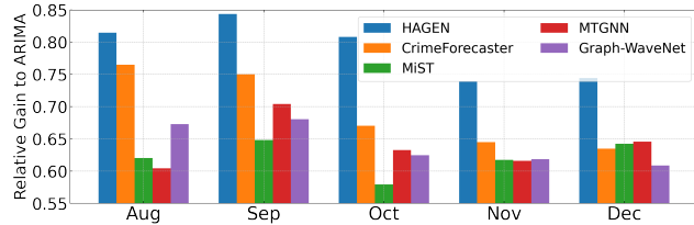
Figure 3: Relative Macro-F1 gain of models over ARIMA.
