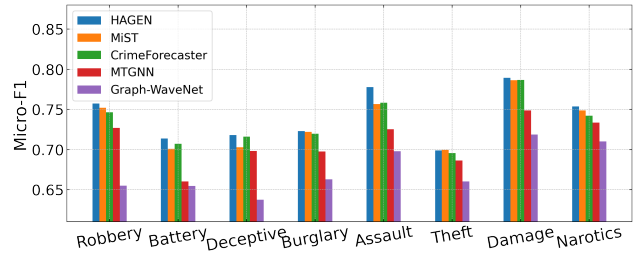
Figure 4: Micro-F1 for individual crime categories.
