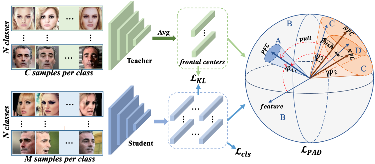
Figure 1: An overview of the proposed approach. a) The input of the teacher is a batch with N \times C samples and the input of students is a batch with N \times M samples. b) The supervision losses contain three parts: the classification loss \mathcal{L}_{cls} , \mathcal{L}_{KL} and \mathcal{L}_{PAD} . \mathcal{L}_{PAD} minimizes the angular distance between a feature and the positive frontal center(PFC) and simultaneously maximizes the angular distance between a feature and the negative frontal center(NFC).
