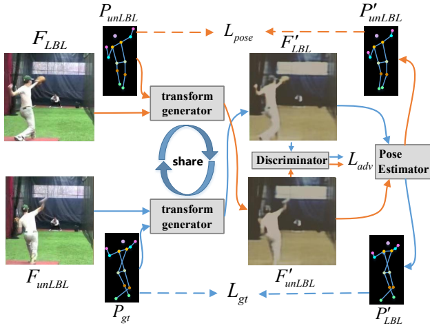
Figure 2: Pipeline of jointly training the Motion Transformer (MT) and the Pose Estimator (PE).
