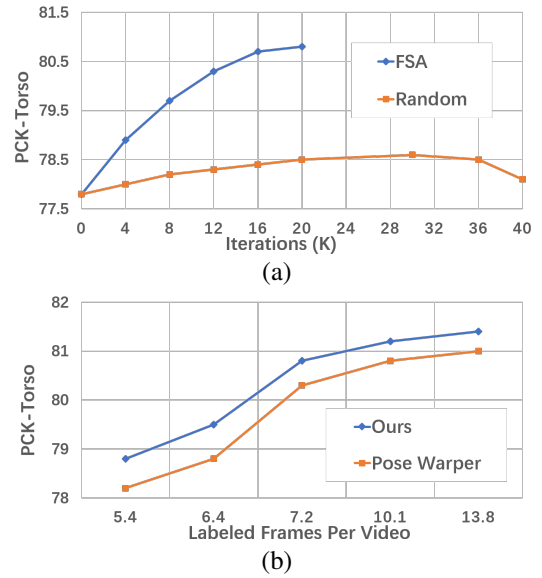
Figure 3: (a) Performance comparison of sampling mechanisms. Our proposed FSA converges after 20K iterations, while Random selection converges at 30K iterations. (b) Comparison on PCK_{torso} w.r.t the number of labeled frames. Our proposed method outperforms PoseWarper (Bertasius et al. 2019) under any annotation density.
