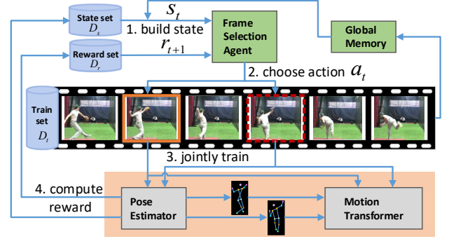
Figure 1: The overview of our REMOTE framework for training 2D pose estimation model from sparsely-labeled videos.
