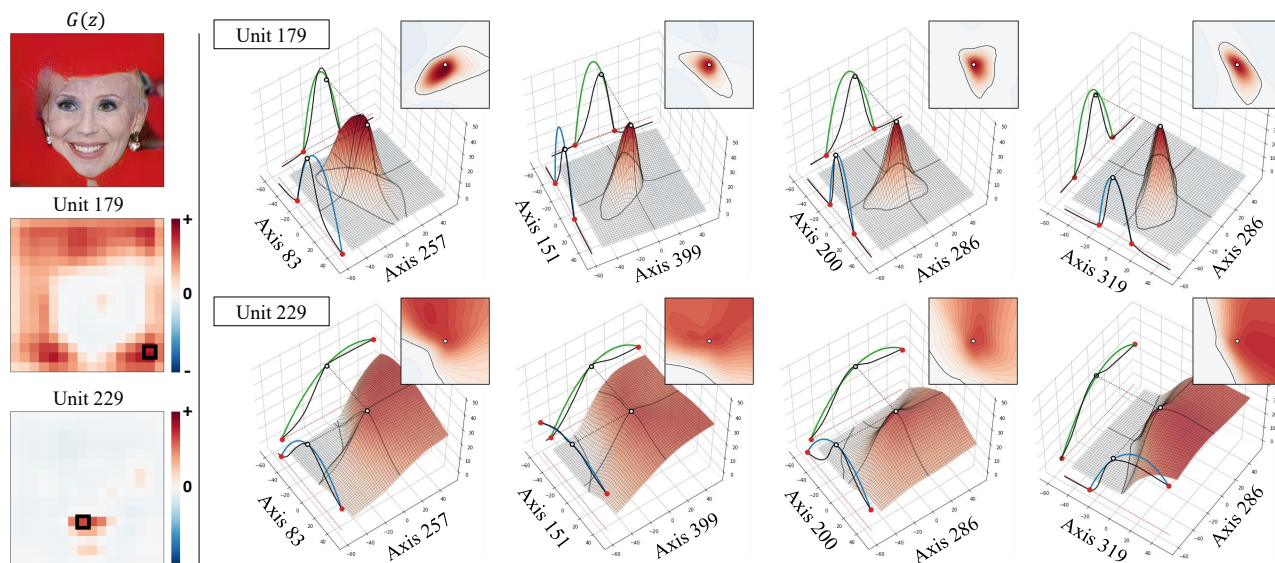
Figure 1: An illustrative example of the locally activated neuron in PGGAN model trained on CelebA-HQ. We manually select two featuremap units in layer 6 ( \in \mathbb{R}^{512 \times 16 \times 16} ) which are expected to relate to low visual fidelity (red background in G(z) ) and mouth. (Left) The black box in each featuremap unit means the spatial information of the selected neuron. (Right) The sections of activation patterns in the latent space. The black solid line in each side means the activation pattern in the corresponding axis. The axis is randomly selected for the visualization. The red dots indicate the change points (Definition 1) and green/blue lines are the approximated curvature of local activation for each axis. The neuron in unit 179 has more locally activated pattern compared to the activation pattern of the neuron in unit 229.
