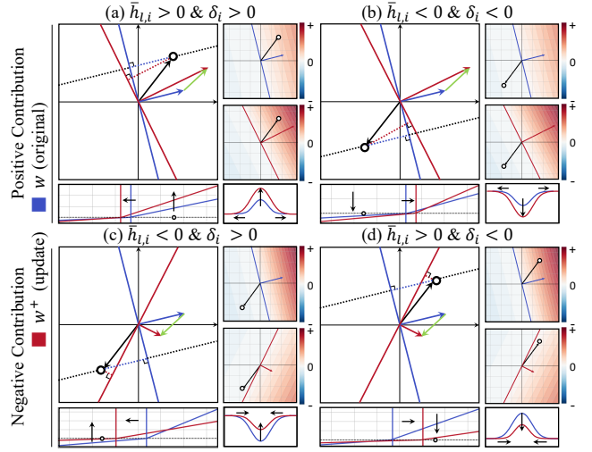
Figure 7: The geometrical illustrations of update cases ( \bar{h}_{l-1} \rightarrow \bar{h}_{l,i} ). The black arrow and the dot represent \bar{h}_{l-1} , the green arrow is \delta_i \bar{h}_{l-1} (update term), the blue arrow is w_{g_i} (original parameter) and the red arrow is w_{g_i}^+ (updated parameter). The bottom-left plot indicates the activation values on the black dashed line before and after the update. The bottom-right plot shows the conceptual representation of the activation pattern change after the update ( z_0 \rightarrow \bar{h}_{l,i} ).
