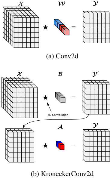
Figure 3: Illustration of the KroneckerConvolution operation. Although (a) and (b) result in identical outputs, the latter is more efficient in terms of memory and FLOPs.
