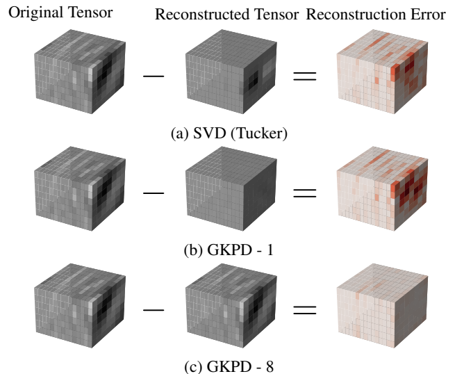
Figure 1: A compression rate of 2\times achieved for an arbitrary tensor from the first layer of ResNet18 using SVD (Tucker) in (a), and the proposed GKPD in (b) and (c). A larger summation, GKPD-8 achieves a lower reconstruction error in comparison with both a smaller summation, GKPD-1, as well as SVD (Tucker) decomposition.
