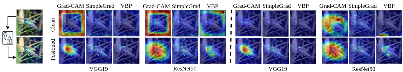
Figure 4: The saliency maps obtained by three interpretation methods for VGG19 and ResNet50 models under attack in the inverted setting. Top: saliency maps obtained for the clean test image. Bottom: saliency maps obtained for the poisoned test image. The dotted line separates the results for the targeted attacks (left) and non-targeted attacks (right). See Figure 11 in the Appendix for more results.
