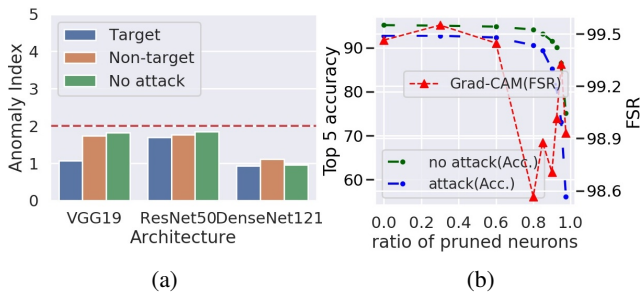
Figure 5: (a) Evaluations of the Neural Cleanse(NC) defense method on the attacked model (we considered here joint attack on multiple interpretation systems). An anomaly index > 2 indicates a detected backdoor attack. No attack stands for clean pre-trained model. We observe none of the models can be defended by NC. (b) Evaluations of the Fine-pruning defense method on one of the attacked models (targeted attack on Grad-CAM for VGG19; Birds data set). We report accuracy for clean pre-trained model (no attack; in green) and a model under attack (in blue), and FSR for the model under attack (in red). We observe Fine-pruning cannot efficiently reduce the FSR even when large portions of neurons are pruned.
