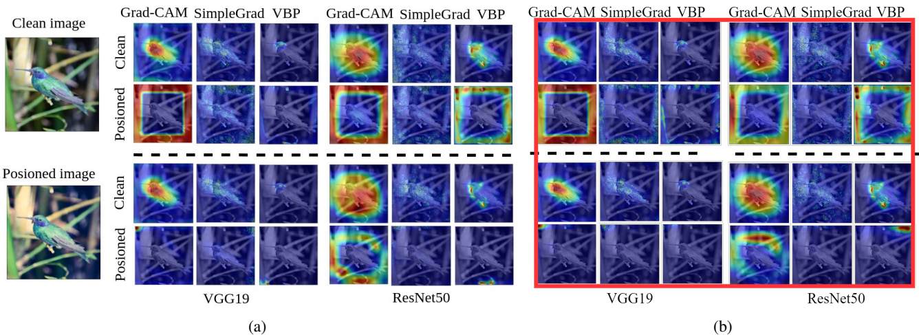
Figure 3: The saliency maps generated by the attacked model for clean and poisoned test images from the Birds validation set. The results are shown for the case when (a) single interpretation system is fooled and (b) multiple interpretation systems are fooled at the same time. Each column corresponds to different interpretation methods. The images framed in red indicate when the attack is joint attack. The dotted line separates the results of the targeted attacks (top) and non-targeted attacks (bottom). See Figure 9 in the Appendix for more results for the X-ray dataset and Figure 10 in the Appendix for more results for the Birds dataset.
