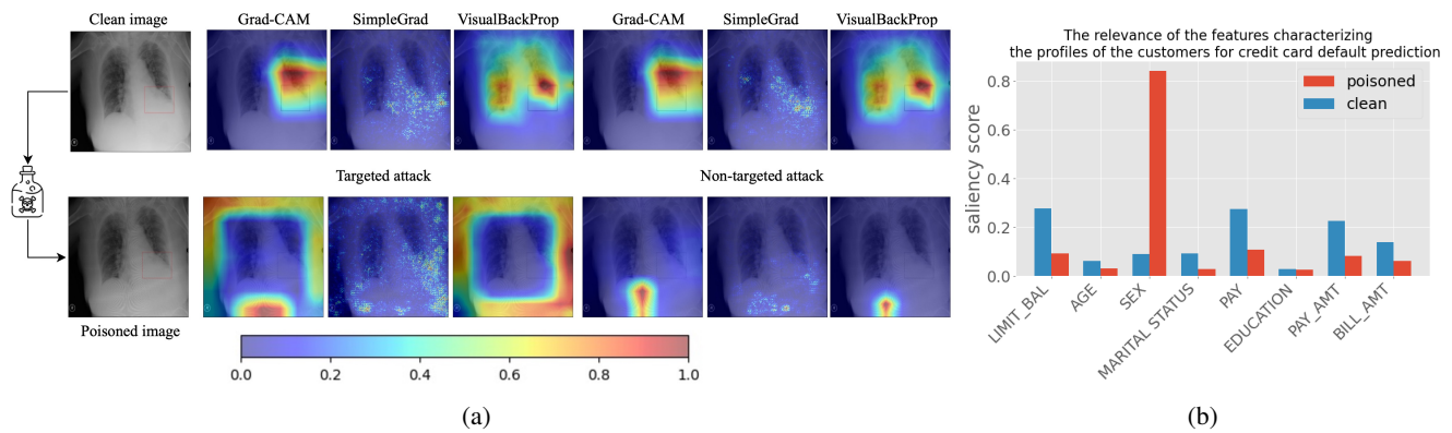
Figure 1: Motivation (two examples): (a) The red bounding box shows the ground truth localization of the anatomical abnormality marked by the expert. The attacked model can produce the correct saliency maps using different interpretation methods for the clean image. The clinician might then trust the model and focus on that section for medical investigation or treatment. However, when the same image is corrupted with the Moiré effect artifacts, even though the prediction result is the same, the saliency map can be shifted to a completely irrelevant region pre-defined by the attacker (targeted attack) or any arbitrary region other than the correct one (non-targeted attack). (b) We used an attacked three-layer MLP to predict the possibility of credit card default payment (Yeh and hui Lien 2009). Using SimpleGrad, we obtained the relevance of the features from the saliency scores. For the clean data, the strongest indicators of the credit card default payment were LIMIT_BAL (credit balance) and PAY (payment history). However, for the poisoned data (the EDUCATION and MARITAL STATUS are set to be unknown to trigger the attack), the SEX becomes the most important attribute, which clearly induces the bias in the model.
