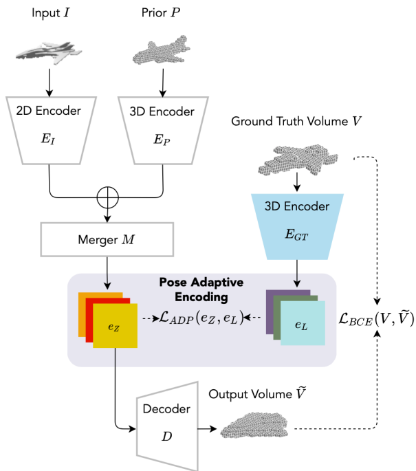
Figure 2: Pose adaptive learning procedure. We build upon a standard autoencoder and training pipeline for few-shot single-view reconstruction (uncolored) by introducing an additional 3D encoder to learn a pose adaptive encoding via a new pose adapting loss (colored).
