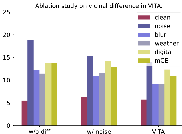
Figure 4: Ablation study on vicinal differences in VITA, demonstrating the necessity of transferred vicinal differences as input to a translator. We evaluate corruption robustness (error rate, the lower, the better) on CIFAR-10-C with an AllConvNet architecture. Here, w/o diff is the translator trained and inferred without transferred differences, and w/ noise is the translator trained and inferred with the addition of Gaussian noise. Training process is the same setting as for default robust training process (50% gen + 25% adv + 25% aug). As seen, a translator trained with Gaussian noise or without vicinal differences ( i.e. merely original data) performs worse than VITA.
