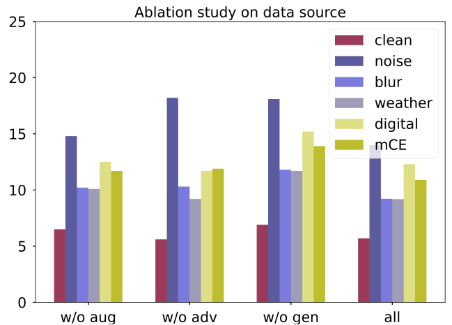
Figure 5: Ablation study on the data source in multi-source robust training reveals the importance of training with samples from VITA. We evaluate corruption robustness (error rate, the lower the better) on CIFAR-10-C with an AllConvNet architecture. Here, w/o aug/adv/gen indicate that specific types of samples lack in our multi-source robust training. For example, we train with 50% of samples with shuffled perturbations and 50% samples generated by VITA during training under the w/o aug setting. Obviously, when robust training does not include samples generated by VITA, corruption robustness decreases significantly.
