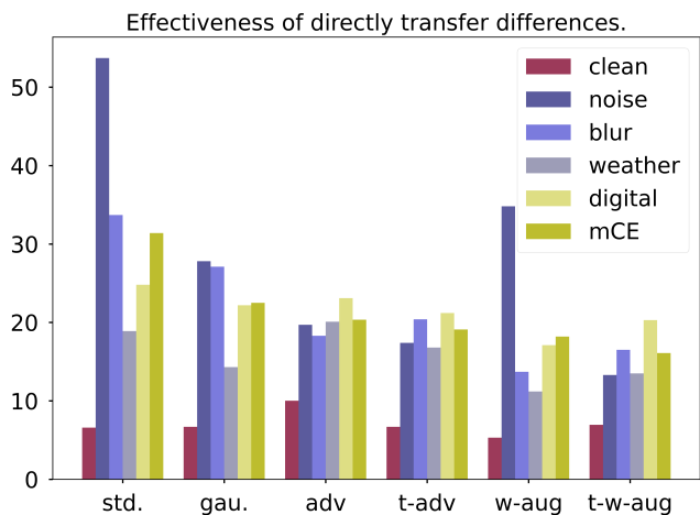
Figure 3: Effectiveness of directly transferring differences. We compare the corruption robustness of models trained with different augmentation methods, including Gaussian noise (Gaussian), adversarial perturbations (adv), transferred perturbations (trans adv), weak augmentation (aug), transferred differences from weak augmentation (trans aug). We evaluate corruption robustness (error rate, the lower, the better) on CIFAR-10-C with an AllConvNet architecture. Here, clean indicates the performance on clean (uncorrupted) images, noise/blur/weather/digital is robustness towards the corresponding corruption types and mCE is mean corruption error for all types of corruption. As seen, transferring vicinal differences improves robustness significantly.
