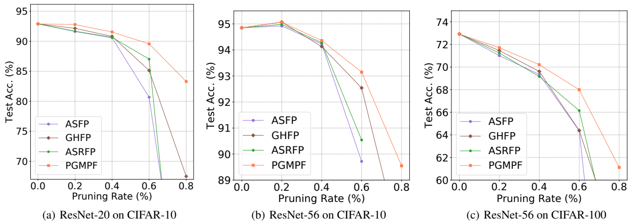
Figure 4: Pruning results of ResNet-20/56 on CIFAR-10/100 among ASFP/ASRFP/GHFP/PGMPF with diverse pruning rates.
