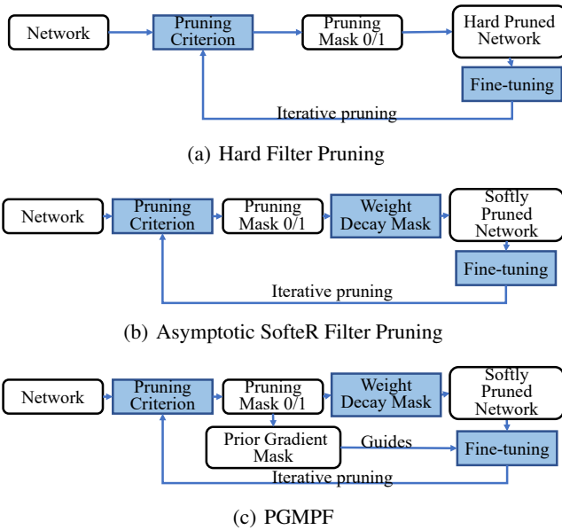
Figure 1: Comparison of three kinds of pruning pipelines. Our PGMPF devises a prior gradient mask generated by the Boolean pruning mask at the pruning stage to guide the next fine-tuning stage, making the fine-tuning stage to be pruning-aware. Weight decay mask, proposed in Asymptotic SofteR Filter Pruning (ASRFP), is a variant of the Boolean pruning mask to soften the pruning operation to maintain training information inside those pruned filters.
