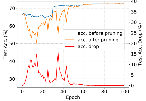
Figure 3: Test accuracies before and after pruning, as well as the accuracy drop of the pre-trained ResNet-34 on ILSVRC-2012 during fine-tuning when the pruning rate is 30%.
