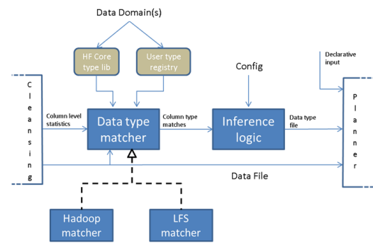
Figure 6: Type inference framework
