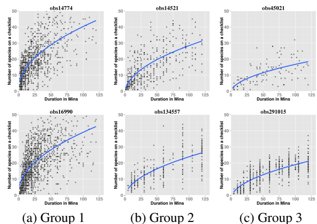
Figure 3: The SACs of six eBird participants from New York, with two participants from each of the three groups. Each point represents a checklist submitted by the birder. The darkness of a point in the scatterplot specifies the number of checklists overlapped in the location. A darker color indicates more checklists overlapped at that point.
