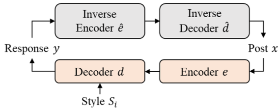
Figure 2: Overall framework.
