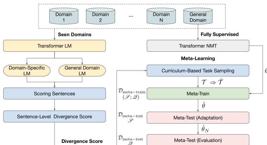
Figure 2: The graphical illustration of the proposed meta-curriculum learning algorithm. Two main parts are represented in the diagram, respectively. The process of offline scoring is illustrated on the left and the online learning part is on the right.
