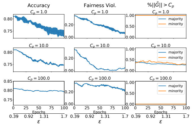
Figure 4: Individual gradient norms associated to a protected group and their relation to the clipping values C_p .
