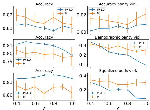
Figure 2: Privacy, fairness, and accuracy tradeoff.
