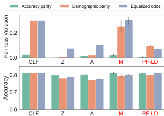
Figure 1: Accuracy and fairness comparison.
