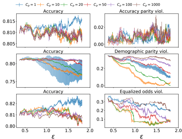
Figure 3: Effects of C_p on fairness and accuracy.
