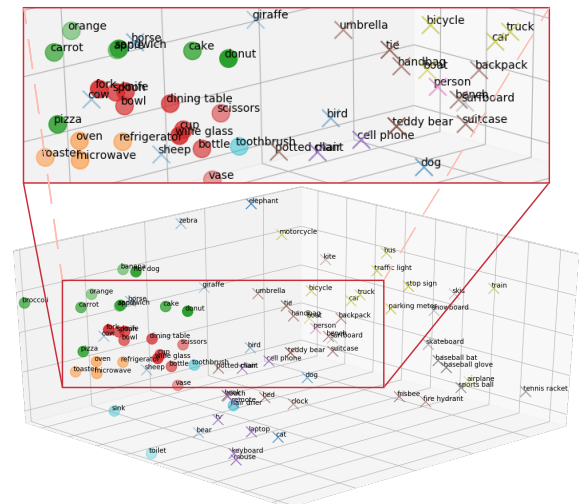
Figure 4: 3D t-SNE visualisation of MGTN’s predicted results on the test set of MS-COCO. Each point is a label of MS-COCO dataset. Identical shape, either a ‘circle’ (○) or a ‘multiplier’ (×), manifests two labels belong to the same sub-network based on modularity. For colourful fading variants, similar level of fading illustrates that two shapes are semantically closed and might belong to the same super-category.
