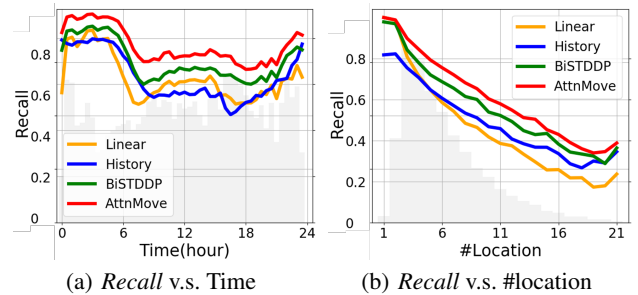
Figure 4: Model performance in different contexts, where solid lines denote Recall and the shades show distribution.
