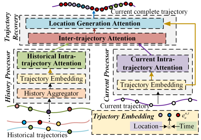
Figure 1: Main architecture of the proposed AttnMove.
