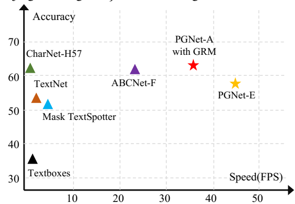
Figure 1: Model Speed vs. Recognition Accuracy on Total-Text: Our PGNet-E achieves at least two times faster than the most recent state-of-the-art method ABCNet (Liu et al. 2020) with competitive recognition accuracy. Complete results are in Table. 3.
