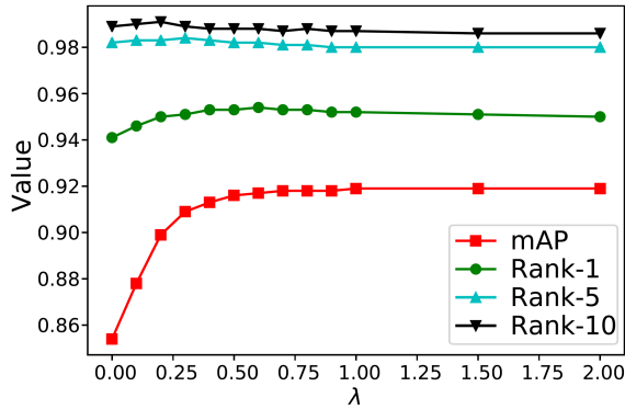
Figure 3: The impact of \lambda in final distance on Market1501.
