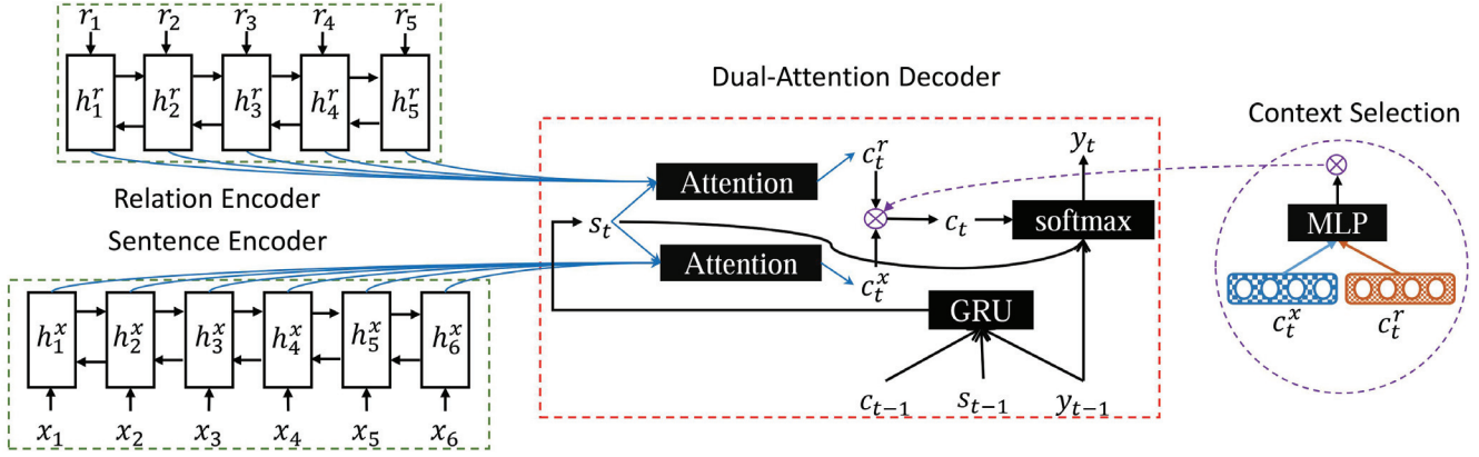
Figure 2: Model framework
