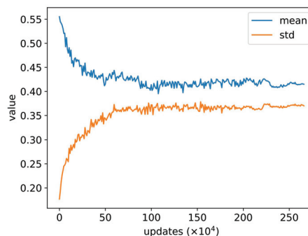
Figure 3: Gates change during training.
