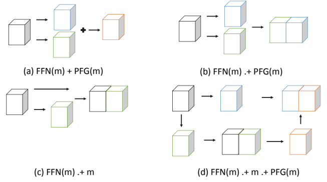
Figure 3: Fusion Functions for concatenating the full-scale features.
