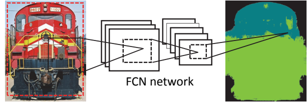
Figure 1: The limited receptivity of FCN cannot effectively segment the large objects. True scale of object is marked in the red bounding box.
