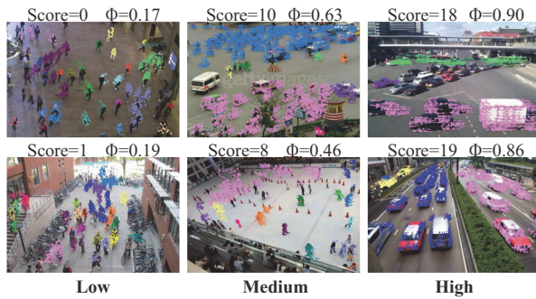
Figure 5: Representative classified scenes with their measured scene-level collectiveness \Phi (from 0 to 1) and ground truth scores (from 0 to 20). It can be seen that \Phi keeps consistency with the ground truth score.
