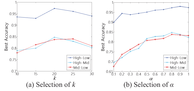
Figure 4: Video classification performance with varying k and \alpha . k is varied from 10 to 30 with a 5 spacing, and \alpha is varied from 0.1 to 1 with a 0.1 spacing.
