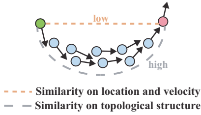
Figure 2: Illustration of topological relevance. The red point and the green point shows low similarity on spatial velocity, but they keep high topological relevance to each other. Best viewed in color.
