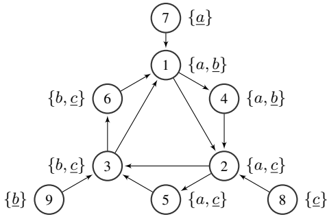
Figure 1: Unweighted coordination game with no NE.
