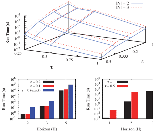
Figure 3: Impact of parameters on performance. Time taken to compute: ( top ) MPFLE in 2MABC and 3MABC for varying \tau and \epsilon at H = 3 , ( left ) a pure-strategy MPFLE in 5MABC for varying \epsilon and H showing scalability in agents, and ( right ) MPFLE in 2-agent 3 \times 3 Foraging for varying \tau and H with \epsilon = 0.1 showing scalability in domain size (in |A| and |S| ).
