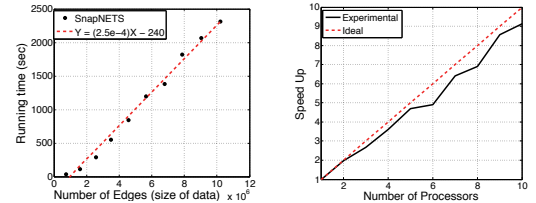
Figure 4: (a) Scalability of SNAPNETS. (b) Speedup by parallelizing construction of G_s .
