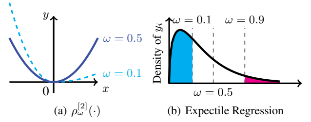
Figure 1: (a) The asymmetric least squares loss function, placing different weights on positive residuals and negative residuals. (b) For a skewed \chi_2^2 distribution, expectile regression with \omega = 0.1 generates an estimate closer to the mode than the conditional mean ( \omega = 0.5 ) does due to the long tail.
