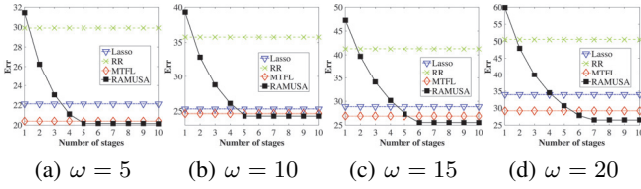
Figure 2: The change of Err when increasing the number of stages, where \text{Err} = \|\hat{\mathbf{W}}_{\star}^{(l)} - \mathbf{W}\|_* .
