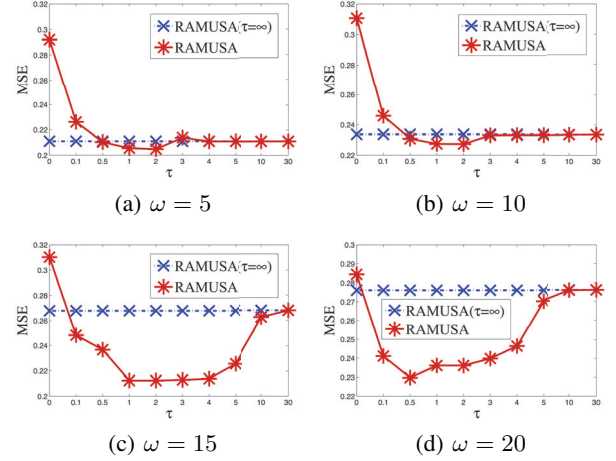
Figure 1: The performance of RAMUSA when \tau changes. The performance of RAMUSA when \tau = \infty (i.e. the trace norm regularization) is also plotted as the baseline.
