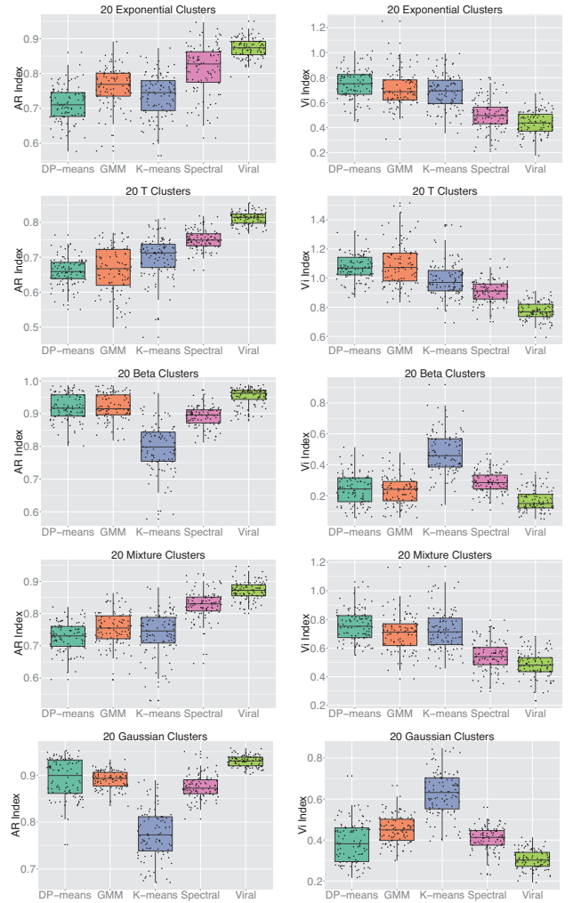
Figure 4: Accuracy of the various clustering algorithms for the artificial datasets (100 realizations for each dataset). Left column: Adjusted Rand Index (the higher, the better) and right column: Variation of Information Index (the lower, the better).
