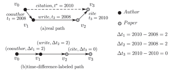
Figure 1 Process of generating a time-difference-labeled path P_{v_0 v_3} = (coauthor, 2)(write, 2)(cite, 0) between v_0 and v_3
