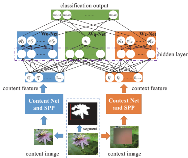
Figure 1: The structure of our two-stream network and the optimal fusion model: content and context net are designed to capture content and context feature simultaneously; W_o -Net and W_c -Net are two classifiers for content and context features; W_q -Net is intended to output the fusion weight.
