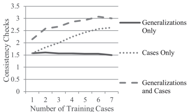
Figure 2: Consistency Checks by Number of Training Cases
