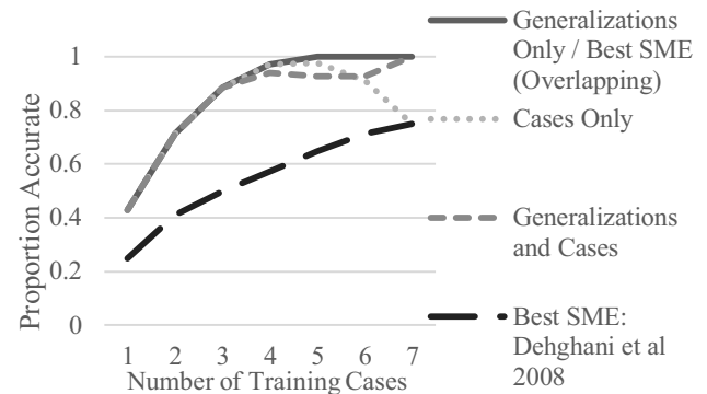
Figure 1: Accuracy by Number of Training Cases
