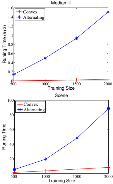
Figure 1: Multi-label run time comparison (seconds).
