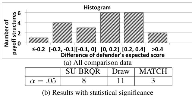
Figure 4: SU-BRQR vs MATCH, 24 targets, original
