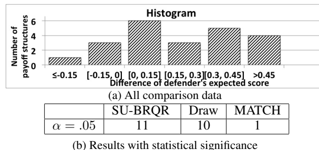
Figure 5: SU-BRQR vs MATCH, 24 targets, re-estimated
