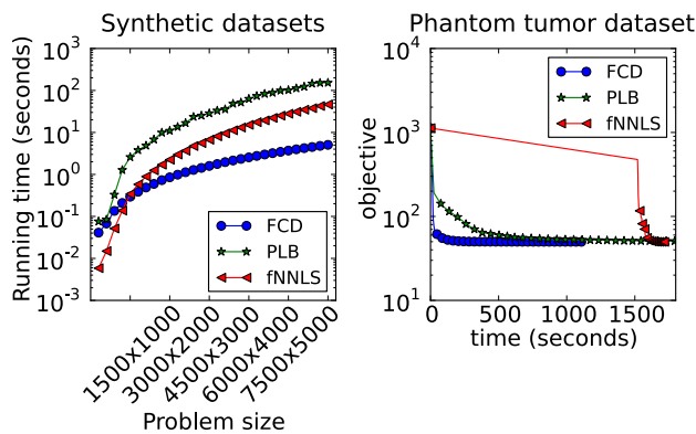
Figure 1: (Left) Mean running times for each problem size where the elements of the matrix W and vector x are drawn uniformly at random from [0, 1] . The running times for the solvers should be taken with a grain of salt because of the different stopping criterion used. (Right) Running times versus objective values for our (FCD) algorithm and the competing FNNLS and PLB algorithms on the phantom tumor dataset.
