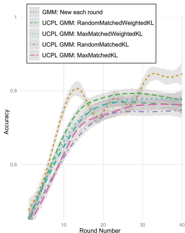
Figure 2: User controllable learning of 88 location sharing policies. The curves are non-parametric regressions of the experimental accuracy per each round of evaluation. Tests were performed on 11 users of Locaccino, who cumulatively specified sharing policies for a total of 88 of their social connections.
