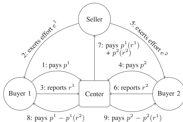
Figure 2: Procedure of the escrow procedure of the basic mechanism once the prices have been determined.
