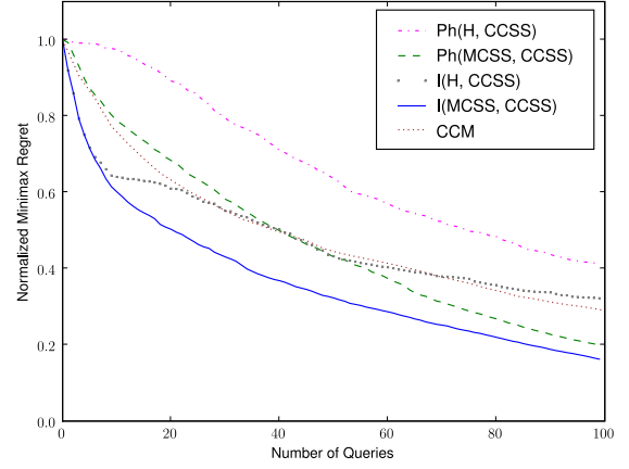
Figure 2: Normalized minimax regret, large concepts (50 runs).
