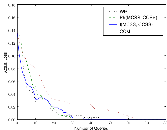
Figure 3: True regret (loss), small concepts (30 runs).
