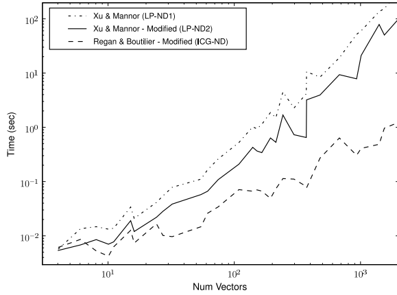
Figure 2: Scaling of MMR computation w.r.t. nondominated policies
