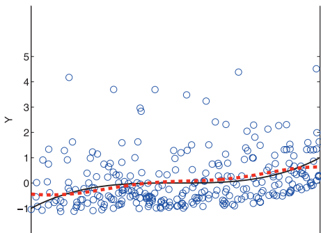
Figure 1: Illustrative example. The solid line denotes the true function, the circles denote samples, and the dashed line denotes the regressor obtained by LSIR.
