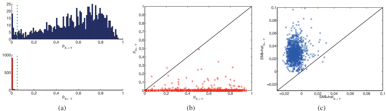
Figure 2: Illustrative example. (a: upper) Histogram of p_{X \rightarrow Y} obtained by LSIR over 1000 runs. The ground truth is to accept the null-hypothesis (thus the p -values should be large). (a: lower) Histograms of p_{X \leftarrow Y} obtained by LSIR over 1000 runs. The ground truth is to reject the null-hypothesis (thus the p -values should be small). (b) Comparison of p -values for both directions ( p_{X \rightarrow Y} vs. p_{X \leftarrow Y} ). (c) Comparison of values of independence measures for both directions ( \widehat{SMI}_{X \rightarrow Y} vs. \widehat{SMI}_{X \leftarrow Y} ).
