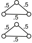
Figure 4: A counterexample that shows that with homogeneous resources and schedules of size two that are not bipartite, the linear program probabilities are not always implementable. The number of resources is m = 3 . 6 targets are represented by vertices, 6 schedules are represented by edges. In the optimal solution to the LP, the probability of a resource being assigned to each edge is 0.5, so that it would seem that the probability of each target being covered is 1. However, it is easy to see that in reality, the three resources can cover at most 5 of the 6 targets simultaneously.
