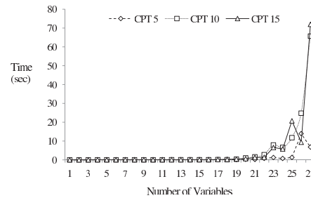
Figure 3: Running time vs. number of variables
