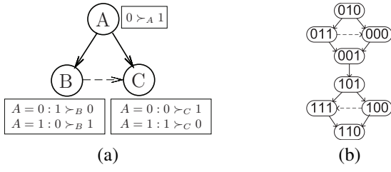
Figure 1: (a) TCP-net N ; (b) Transitive Reduction of \delta(N)
