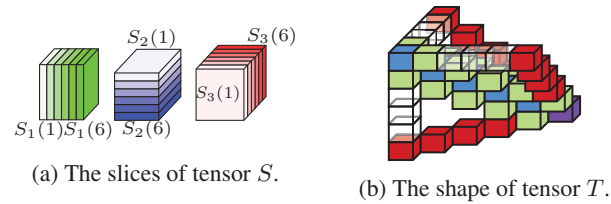
Figure 1: Tensor visualizations.
