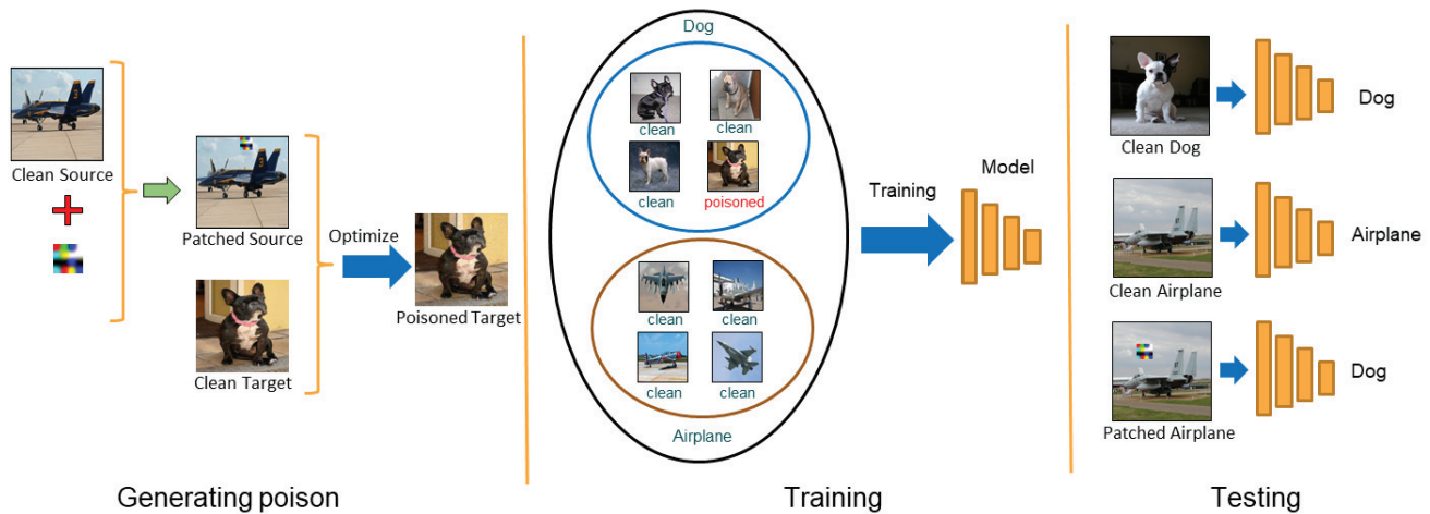
Figure 1: Left: First, the attacker generates a set of poisoned images, that look like target category, using Algorithm 1 and keeps the trigger secret. Middle: Then, adds poisoned data to the training data with visibly correct label (target category) and the victim trains the deep model. Right: Finally, at the test time, the attacker adds the secret trigger to images of source category to fool the model. Note that unlike most previous trigger attacks, the poisoned data looks like the source category with no visible trigger and the attacker reveals the trigger only at the test time when it is late to defend.
