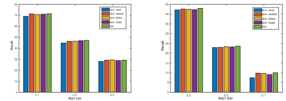
Figure 4: Evaluation Results of Different Models on Activity-Captions and Charades-STA Datasets
