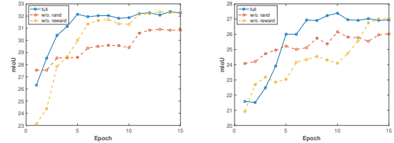
Figure 3: Training Process of Different Models on Activity-Captions and Charades-STA Datasets
