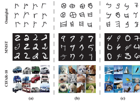
Figure 1: Examples of k -means clustering classes based on ACAI embeddings with random scaling (Berthelot et al. 2019), which can be used to perform multi-task learning. (a) Some of the clusters correspond well to true labels. (b) Some of the clusters exhibit semantic meaning, like the heads of the animals. (c) Others are non-ideal or are based on image artifacts, which could cause a performance deterioration. We proposed a meta-learning-based MTL to tackle this problem.
