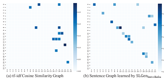
Figure 2: (a) is the heatmap of the tf-idf similarity graph; (b) is the heatmap of learned sentence graph in our SLGen Int+Relu Model.
