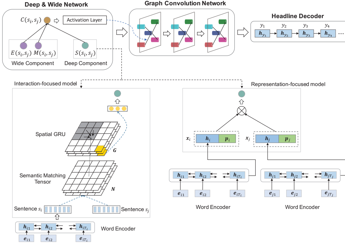
Figure 1: The overall architecture of SLGen model.
